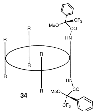
34 R = (R) \text{ NHC(O)C(CF}_3\text{)(C}_6\text{H}_5\text{)(OMe)}
