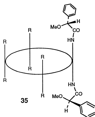
35 R = (R) \text{ NHC(O)CH(C}_6\text{H}_5\text{)(OMe)}
